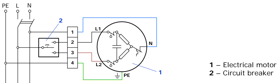
Fig.1 – Electrical interfaces
